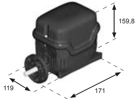
Yankee 1 absolute encoder
